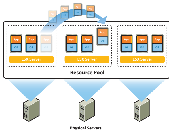
VMware DRS automatically and intelligently balances resources among virtual machines.
